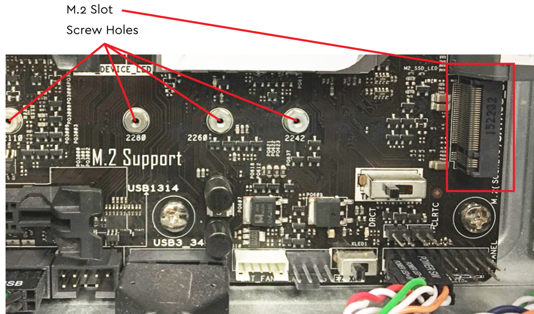
Example of a Motherboard M.2 Mounting Setup
