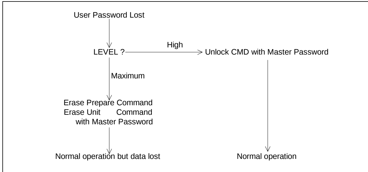
Figure 10 Password Lost
