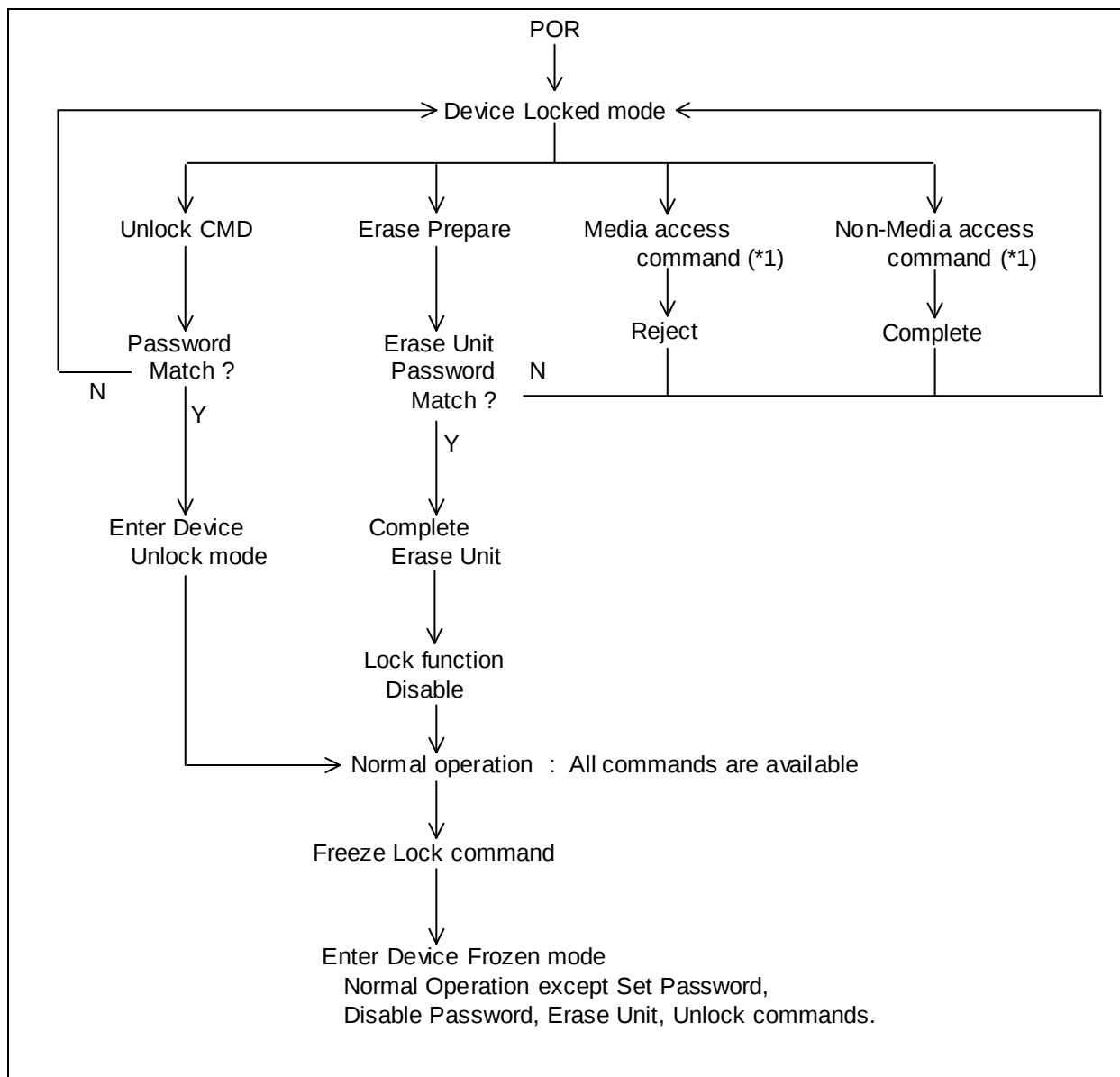
Figure 9 Usual Operation
