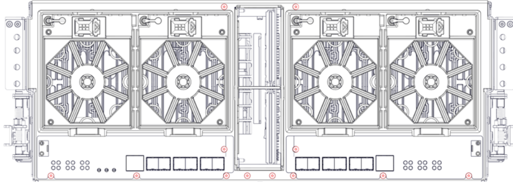
Figure 35: Fan Housing, As Viewed from the Rear
