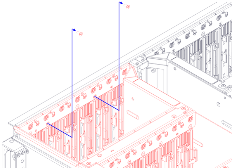
Figure 47: Right-Front Inside Corner, As Viewed from the Right-Rear-Top
