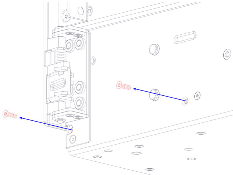
Figure 50: Right-Front Outside Corner, As Viewed from the Right-Rear-Bottom
