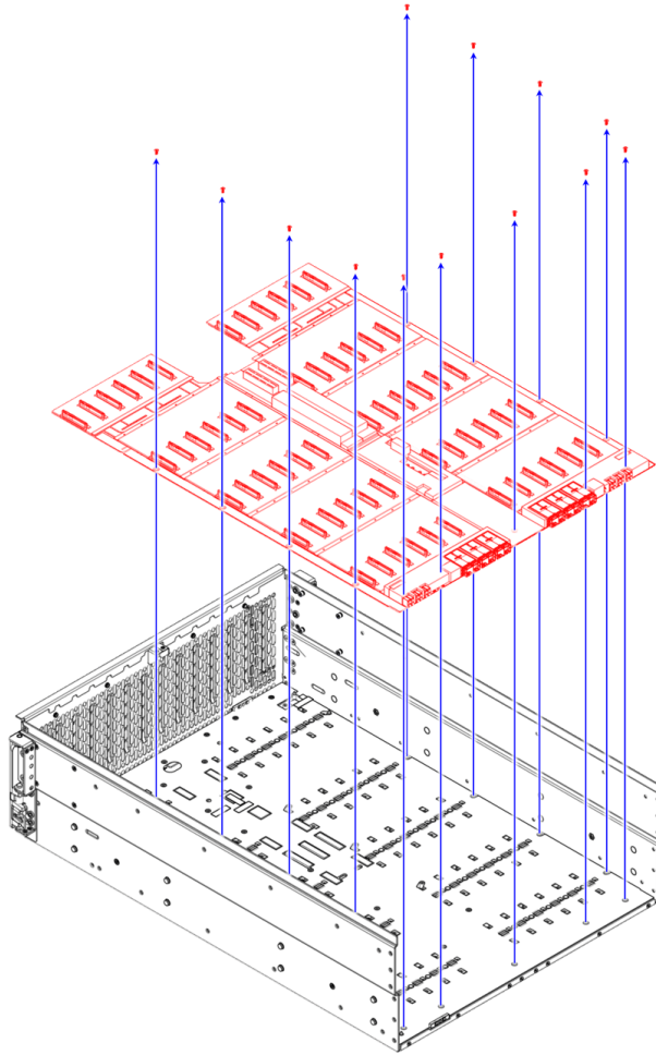
Figure 60: Rear Baseboard, As Viewed from the Right-Rear-Top
