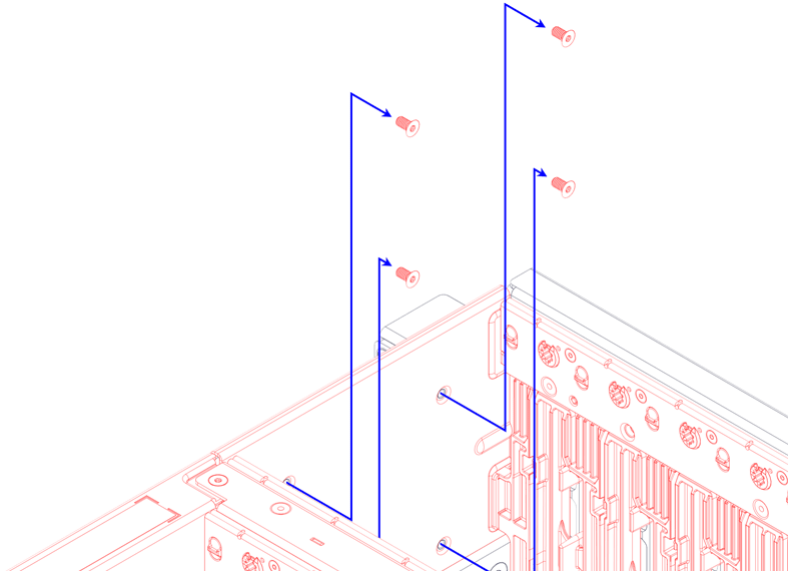
Figure 48: Right-Front Inside Corner, As Viewed from the Left-Rear-Top
