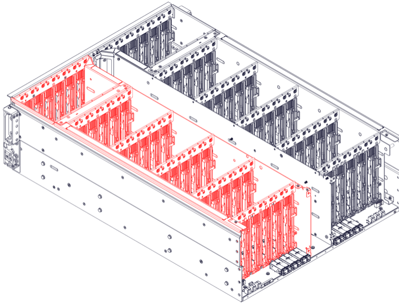
Figure 46: Right Drive Housing, As Viewed from the Right-Rear-Top
