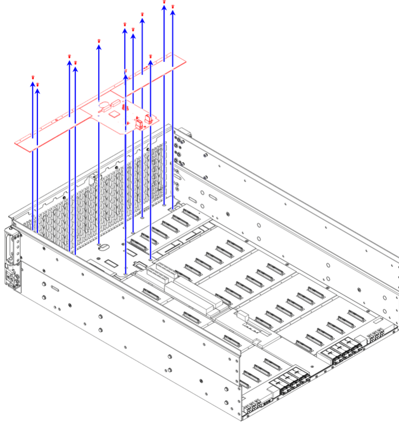
Figure 58: Front Baseboard, As Viewed from the Right-Rear-Top
