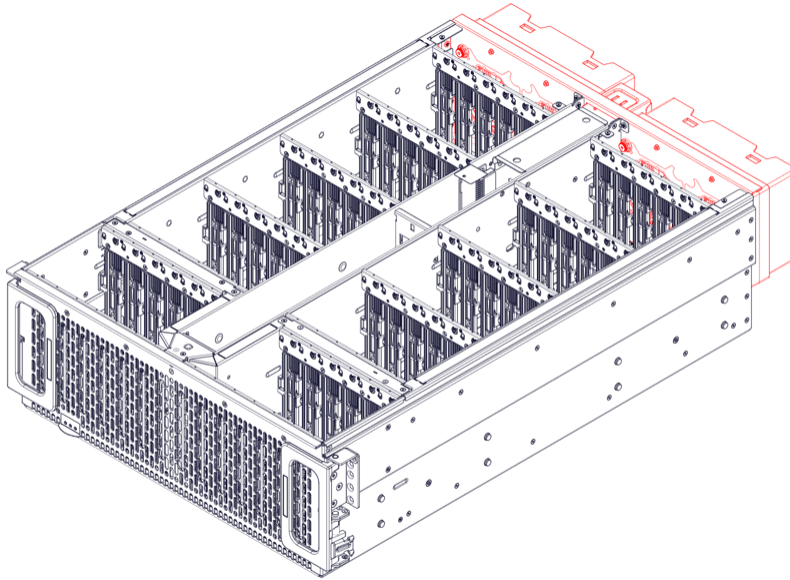
Figure 34: Fan Housing Assembly Location
