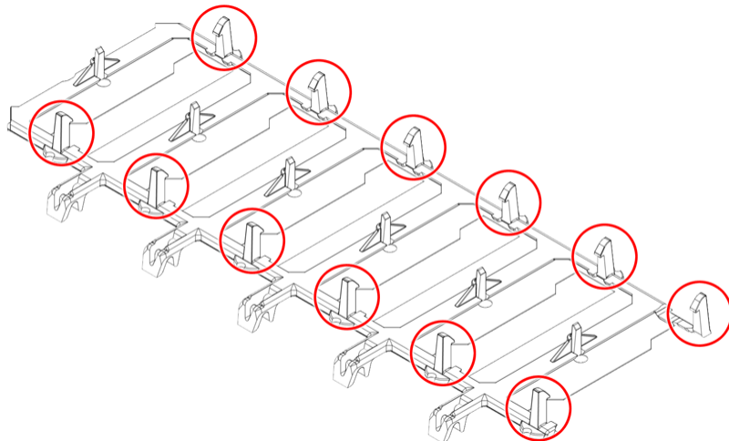
Figure 54: HDD Limiter, Bottom Side Clips
