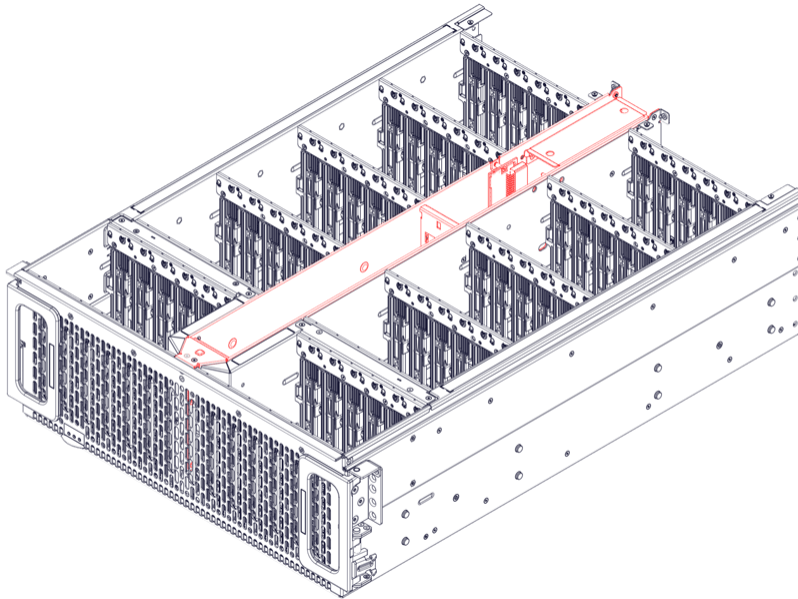
Figure 41: IO Housing Location
