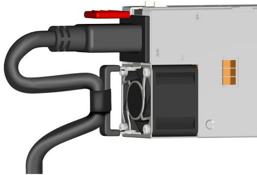
Figure 4: Strap-Style Cable Retention
