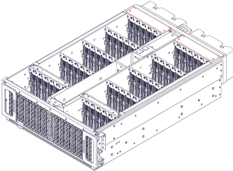
Figure 30: Plenum Covers Location
