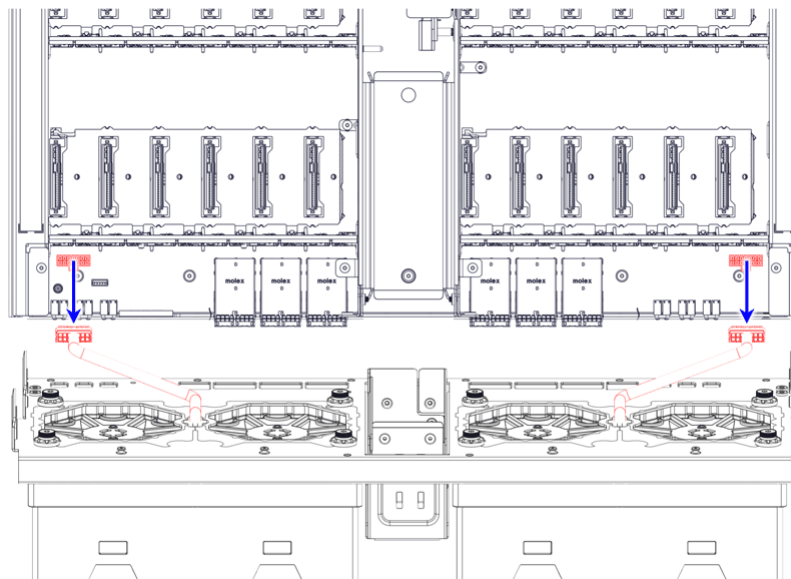
Figure 37: Fan Cable Connectors, As Viewed from the Top-Rear
