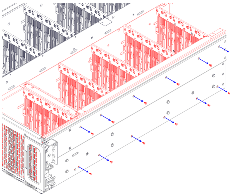
Figure 51: Right-Front Corner, As Viewed from the Right-Front-Top
