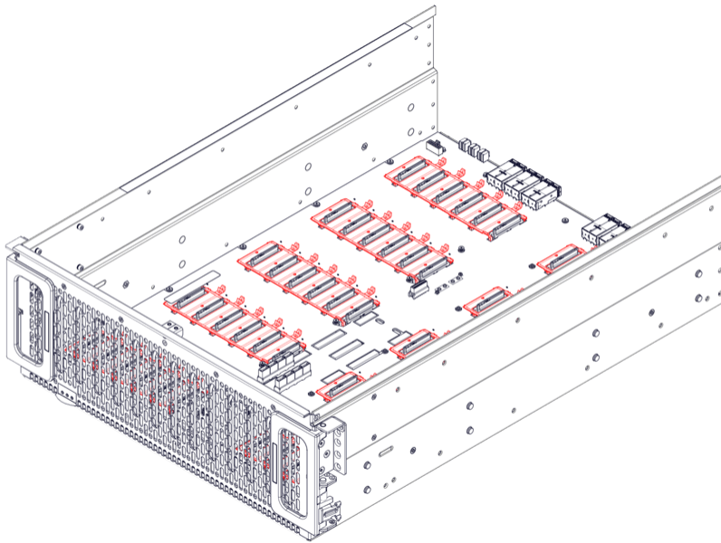
Figure 53: HDD Limiters Location
