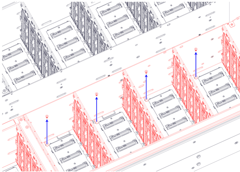
Figure 49: Right Drive Bays, As Viewed from the Right-Front-Top
