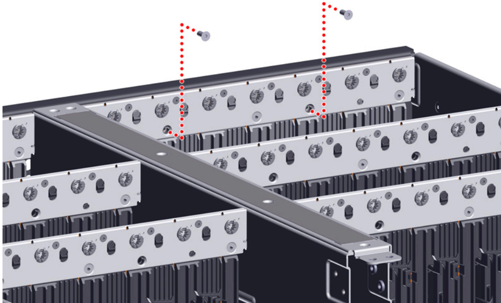
Figure 55: Front-Left Corner, As Viewed from Right-Rear-Top
